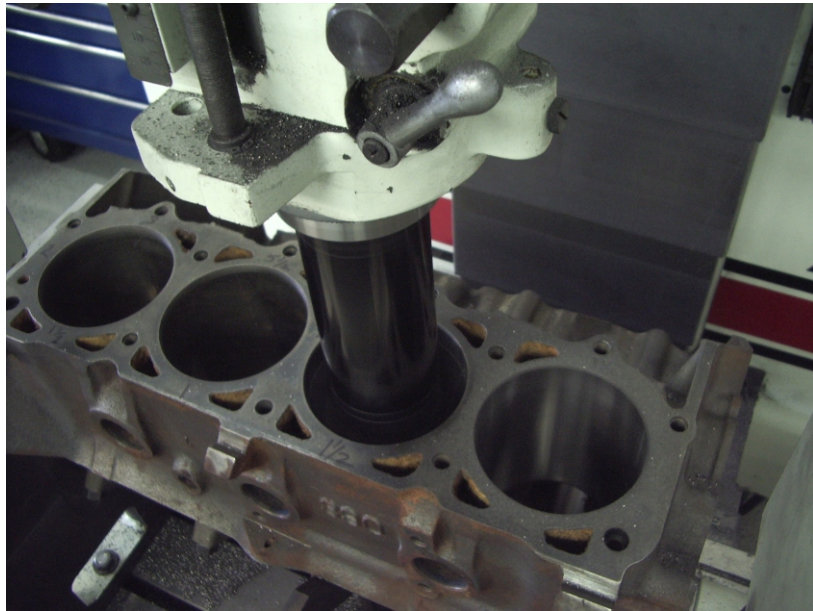
Boring a Cylinder Block
