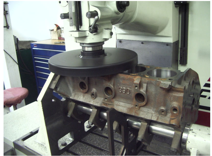
Surfacing a Cylinder Block
