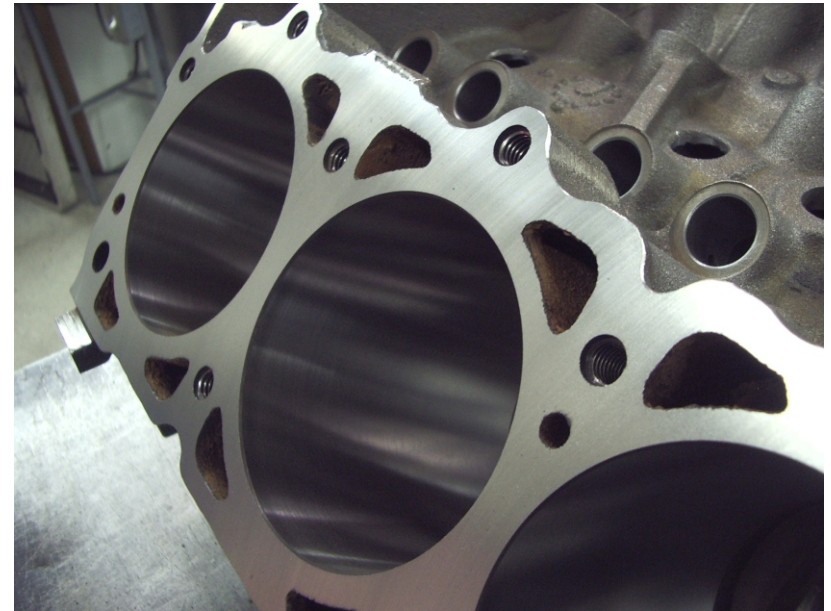
Completed Block Surfaced
